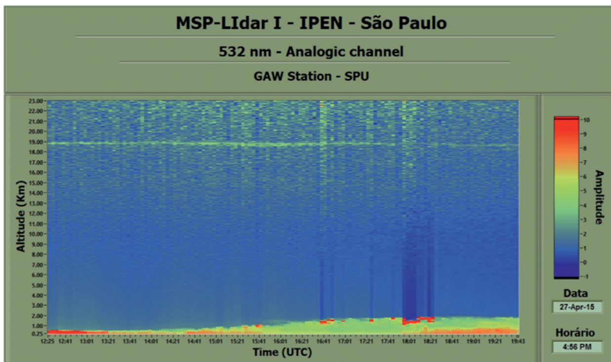
FIG. 12. Lidar RCS at 532 nm measured at SPU (São Paulo, Brazil) the afternoon of 27 Apr 2015. The signal around 19 km is aerosols from the Calbuco volcanic eruption.
