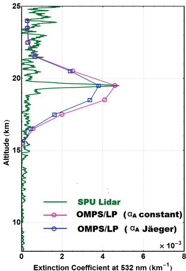
FIG. 13. Lidar aerosols extinction profile at 532 nm (green) retrieved by the SPU (São Paulo, Brazil). OMPS/LP aerosols extinction profiles at 532 nm derived from OMPS/LP aerosol extinction profiles at 674 nm, using two sets of Ångström exponents, indicated here as \alpha_A .
